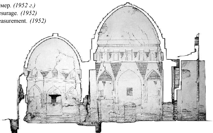
41, 42. Разрез запад – восток. 41, 42. Coupe ouest – est 41, 42. Section from west to east.
