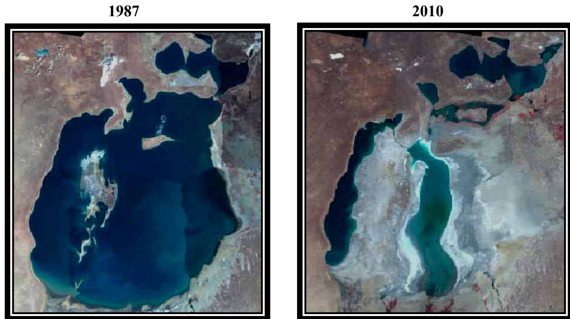
Figure 1 - Aral Sea changes in two time span
