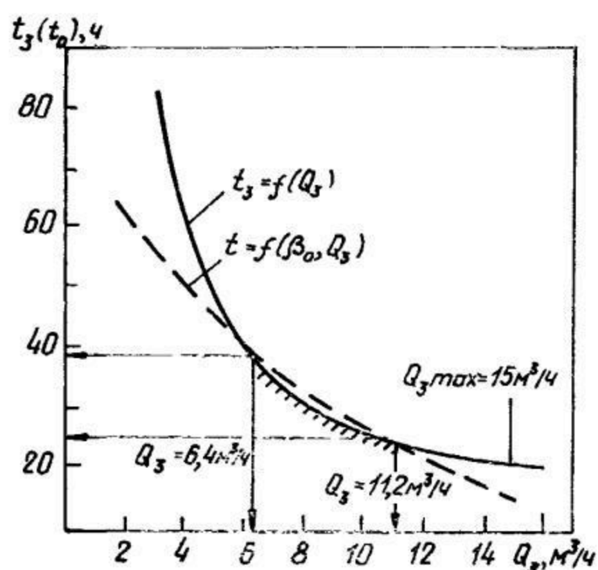
Рис. 21.23. Зависимости t_3 = f(Q_3) и t = f(\beta_0, Q_3)
