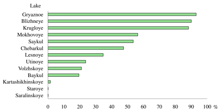
Fig. 2. Degree of lake overgrowth
