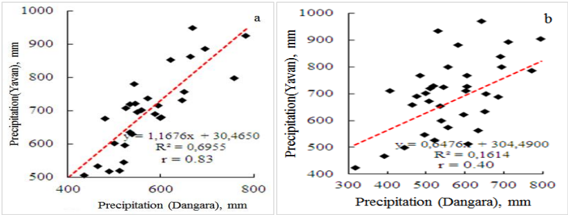
Fig. 9. Correlation of mean annual precipitation in Dangara and Yavan for the periods 1950 - 1979 (a) and 1980 - 2020 (b)
