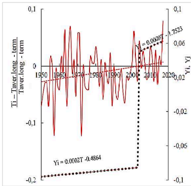
Fig. 6. Ratio of annual mean and annual long-term temperature difference to annual long-term temperature and temperature trend for Yavan district before and after reservoir construction
