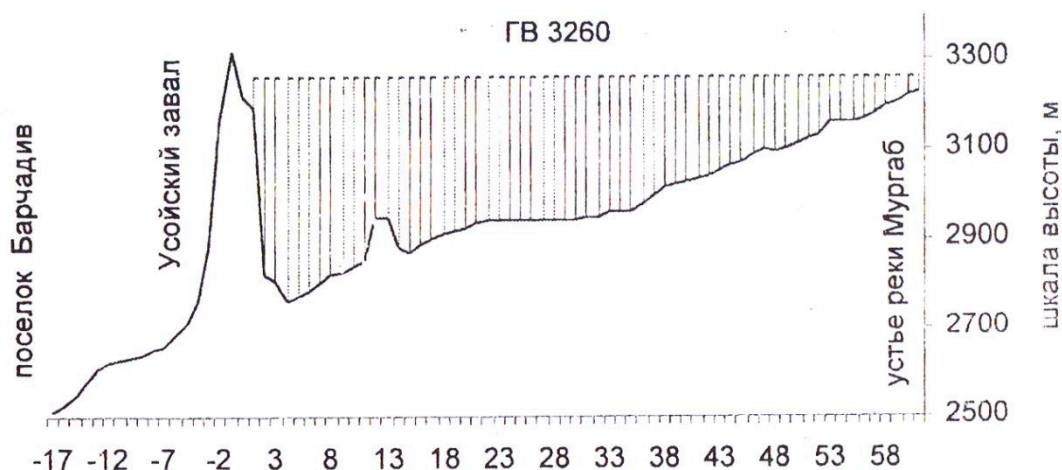
Fig. 8.5 - Longitudinal profile of the Bartang River in the Sarez lake basin
