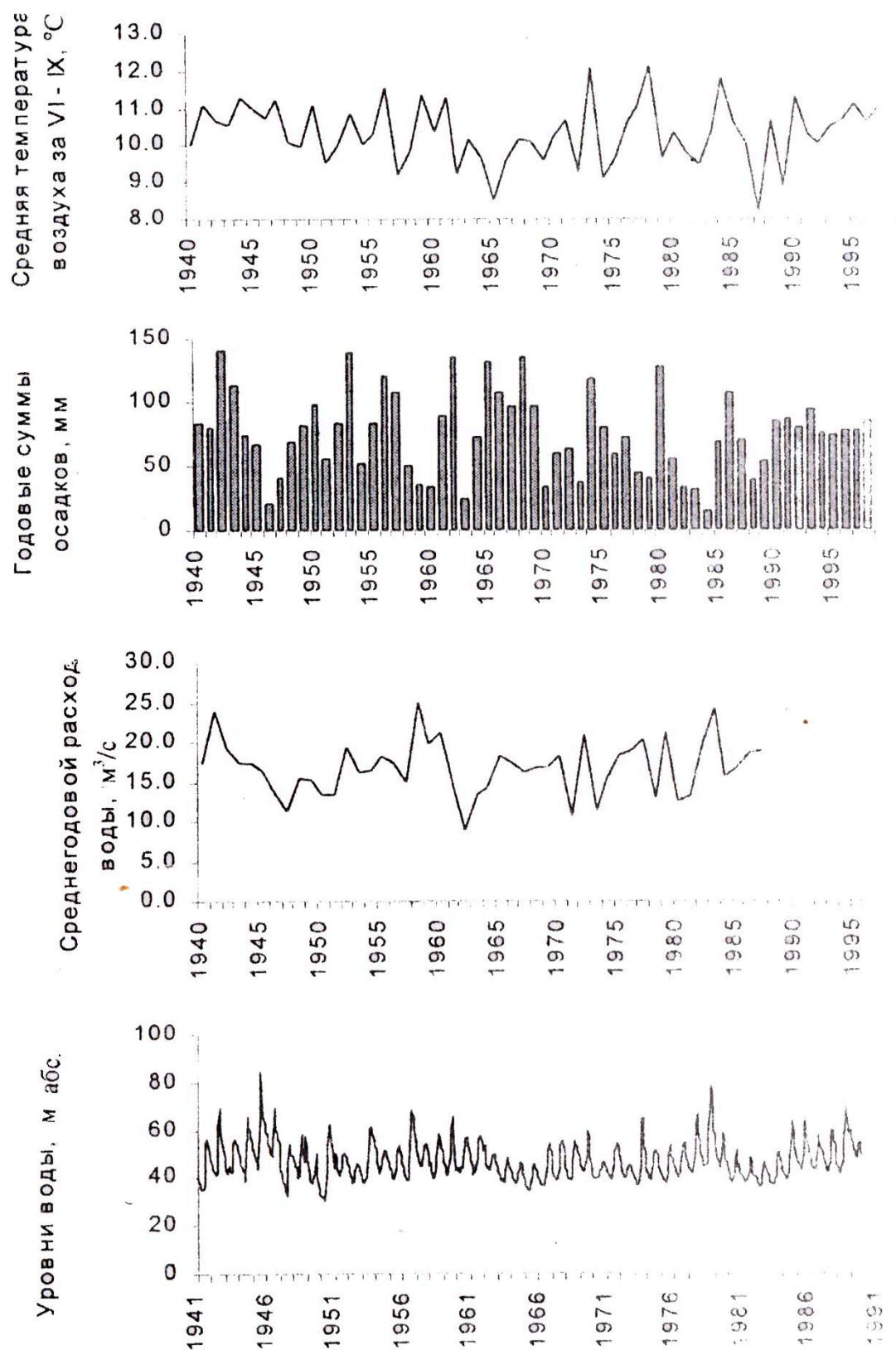
Fig. 8.12 - Long-term changes in the hydrometeorological characteristics of the Sarez Lake basin (by the example of the Lyangar-Ustye River) [11]
